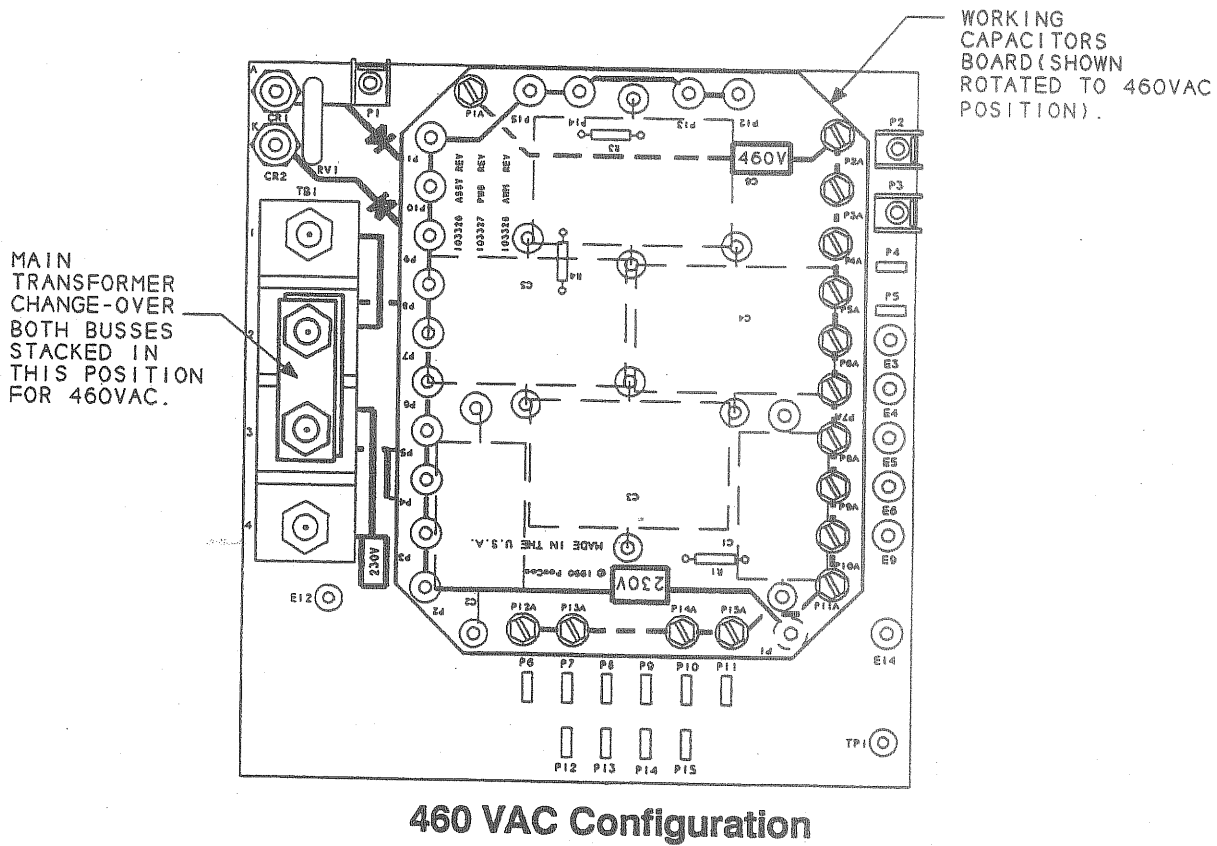
Figure 3, Voltage Change-Over Configurations
